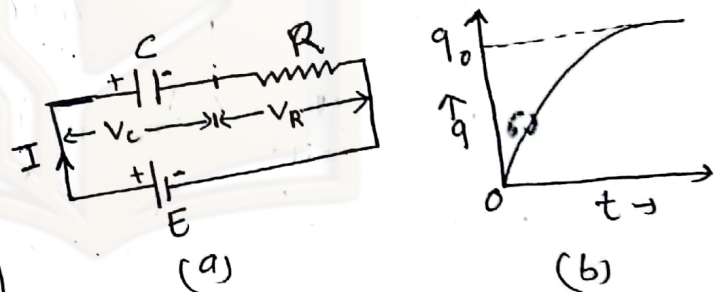
[Fig: (a) charging of a capacitor, (b) graph showing the charging nature of capacitor]
